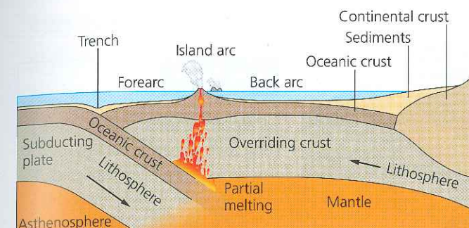
Figure 1.4 Subduction and the development of island arc volcanoes at a destructive boundary
