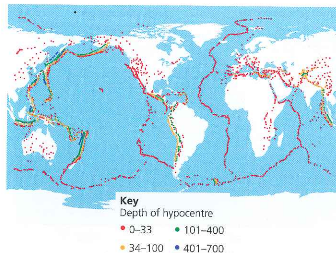
Figure 1.10 Different depth tectonic earthquake boundaries mapped on to a world map
