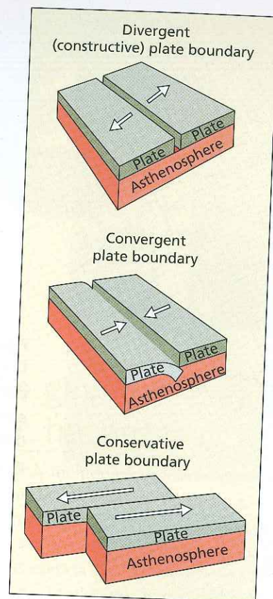
Figure 1.3 Different plate boundaries
