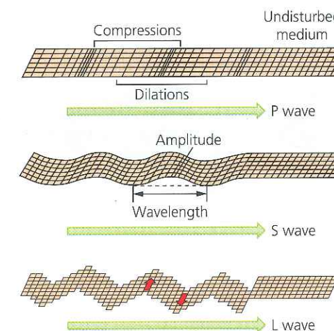
Figure 1.12 Differences between P, S and L waves
