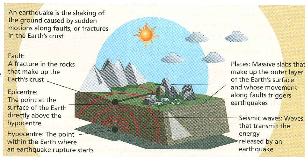
Figure 1.11 Anatomy of an earthquake
